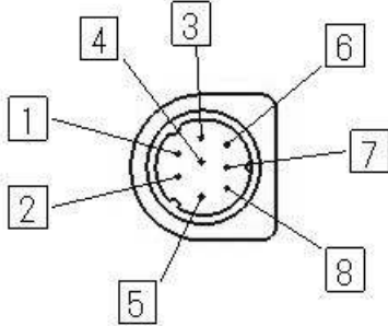
miniDIN 8pin
