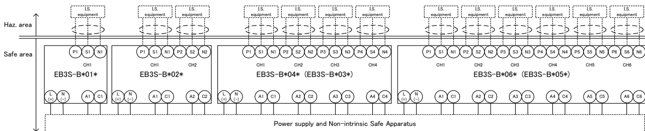
Fig.2 System configuration
