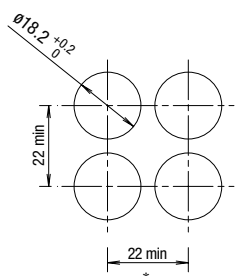
Round (LB6S/LB6MS)
