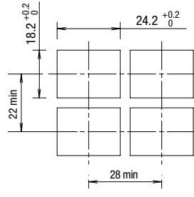
Rectangular (LB8S/LB8MS)
