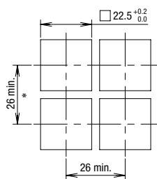
Square (LBW7S/LBW7MS)
