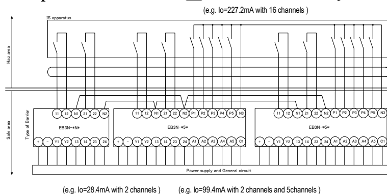
(e.g. Io=28.4mA with 2 channels) (e.g. Io=99.4mA with 2 channels and 5channels)
