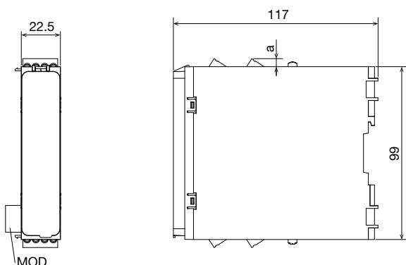
HR6S-EP形
