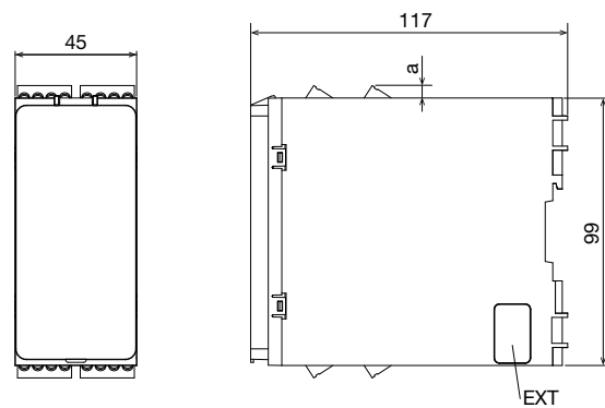
HR6S-AT形
