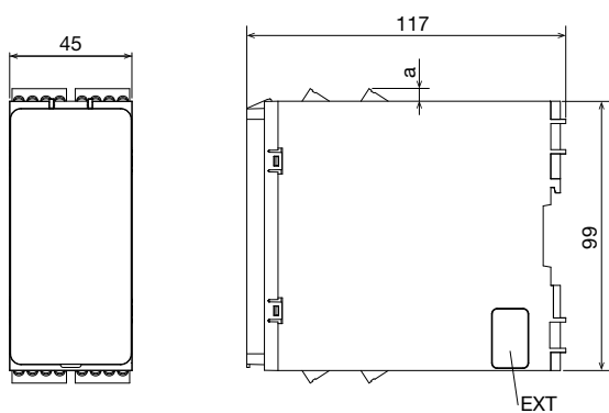
HR6S-DN形
