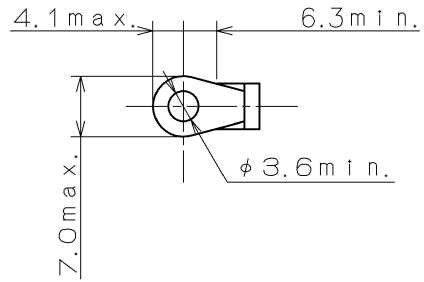
Applicable Crimp Terminal
