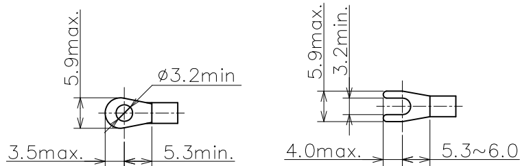
Applicable crimping terminals
